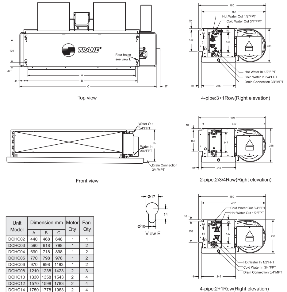
Fig 2: DCHC Without Return Plenum
