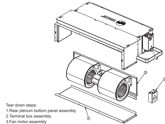
Fig 7: Rear Plenum Unit-Fan Motor Assembly Tear Down
