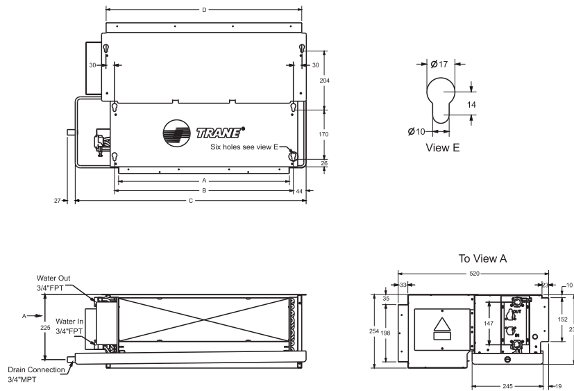
Fig 3: DCHC With Rear Plenum
