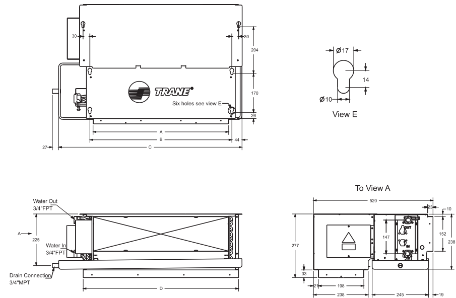
Fig 4:DCHC With Bottom Return Plenum
