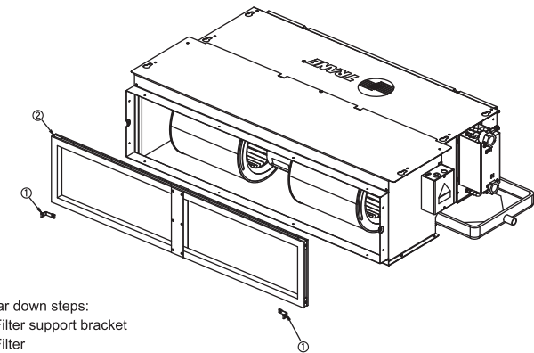
Fig 6: Rear Plenum Assembly-Filter Tear Down (Option)
