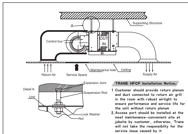
Fig.5: Typical Installation
