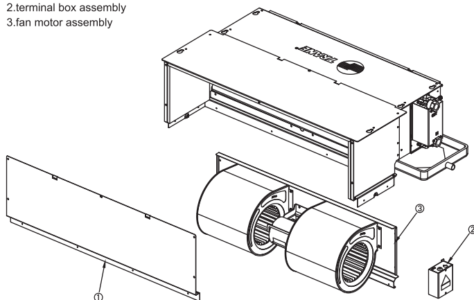
Fig 9: Bottom Return Plenum Unit-Fan Motor Assembly Tear Down
