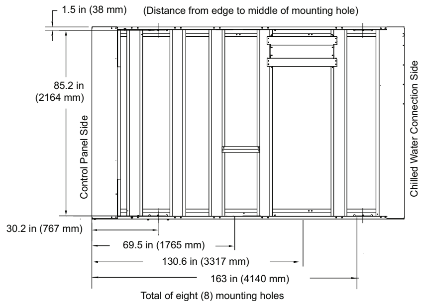
Figure 20. Mounting locations, 130 ton
