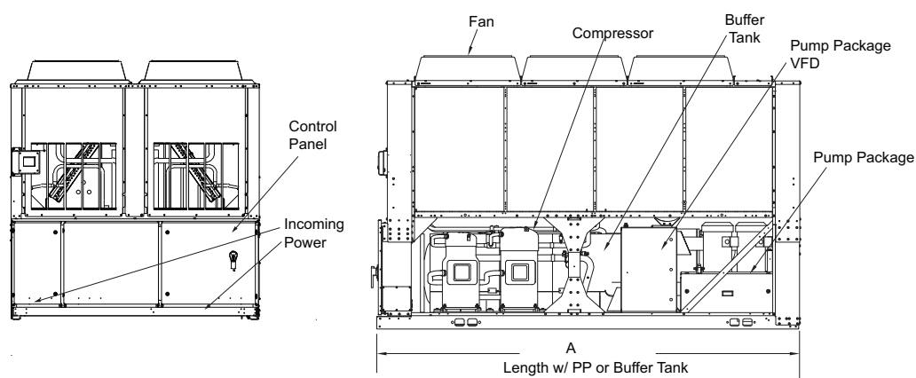
Figure 10. Dimensions, 80 to 120 ton units with options
