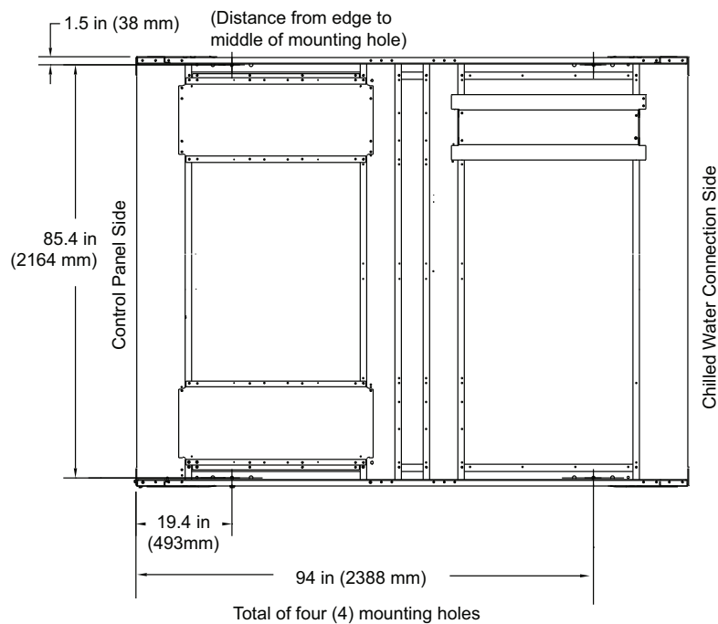
Figure 18. Mounting locations, 60 and 70 ton
