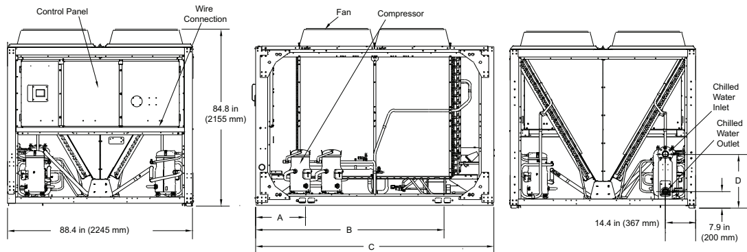
Figure 5. Dimensions, 40 to 70 ton units, no options
