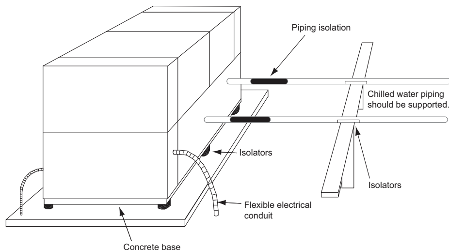
Figure 3. Installation example
