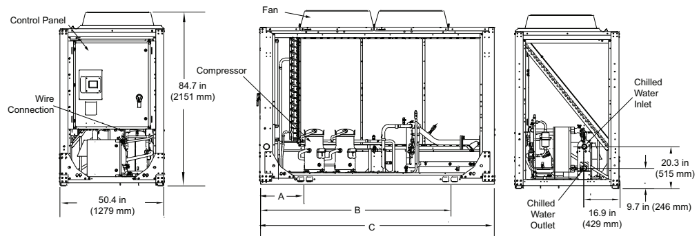
Figure 4. Dimensions, 20 to 35 ton units, no options
